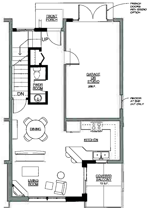
2 TYP. MAIN FLOOR 828 S.F. SCALE: 1/4" = 1'-0"
